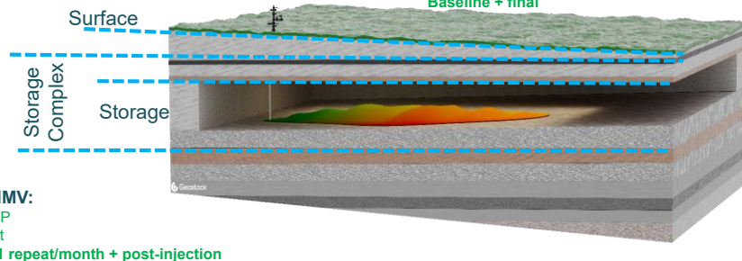
Figure 4.2 Monitored subsystems of the geosphere for a CO 2 injection pilot project in the Paris Basin
