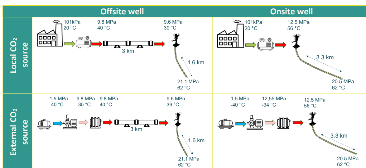
Figure 4.1 Development scenarios considered for a CO 2 injection pilot project in Paris Basin
